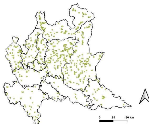
Fig. 7-b – 100 Bq/m 3 < Rn-222 < 200 Bq/m 3
